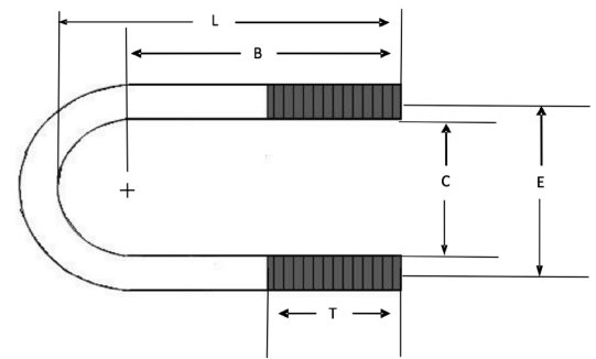
FIGURE 137 U-BOLT DIMENSIONS
